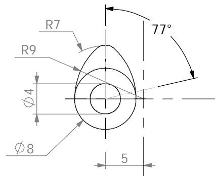
Came
